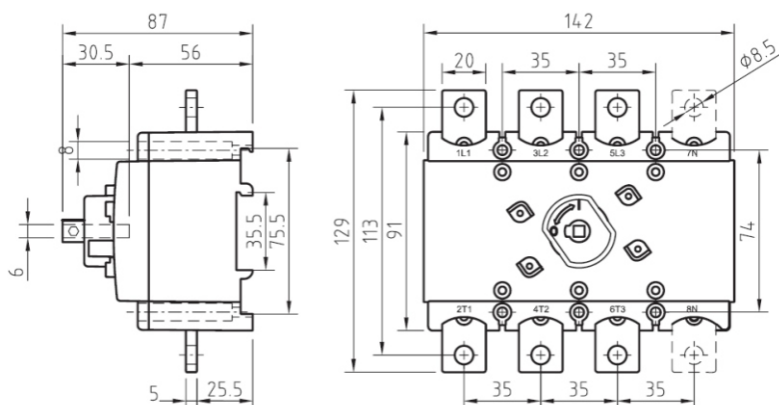
VKA series 250 A (3 pole)
