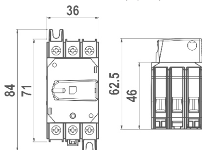
KU3** Series 16 - 40 A (3 pole)
