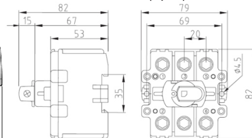
VKA3***N series 125 - 160 A (3 pole)
