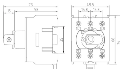
KU3**N Series 63 - 80 A (3 pole)
