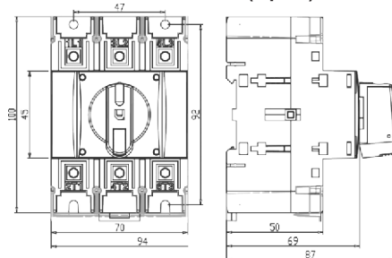
KU3*** series 125 - 160 A (3 pole)
